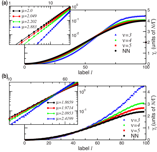
FIG. 3. (Color online) Imaginary parts \gamma_l (symbols) in ascending order for LRI systems with \nu=3, 4, 5 , and for NNIs for N=100 and \Gamma=(a) 0.001 and (b) 1. The inset shows the power-law behavior of the \gamma_l in the intermediate l region with the appropriate exponents \mu .
