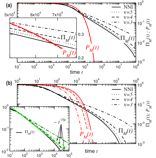
FIG. 1. (Color online) \nu dependence of the quantum mechanical \Pi_M(t) and the classical P_M(t) decay behaviors for a chain of N=100 sites; here \Gamma=(a) 0.001 and (b) 1. The inset in (a) shows a closeup picture of the region where \Pi_M(t) and P_M(t) cross. The inset in (b) shows power-law fits (see arrows) to \Pi_M(t) in the intermediate time regime with exponents 1/\mu , where the \mu are taken from Fig. 3(b).
