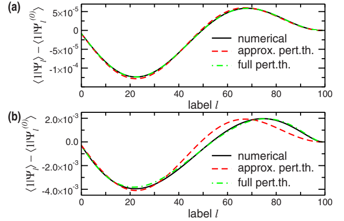
FIG. 2. (Color online) Correction term \langle 1 | \Psi_l \rangle - \langle 1 | \Psi_l^{(0)} \rangle for N=100 and for \nu=(a) 10 and (b) 5. The direct numerical evaluation (solid black line) is compared to the perturbation theory expression Eq. (8) (dash-dotted green line) and to the approximate expression Eq. (9) (dashed red line).
